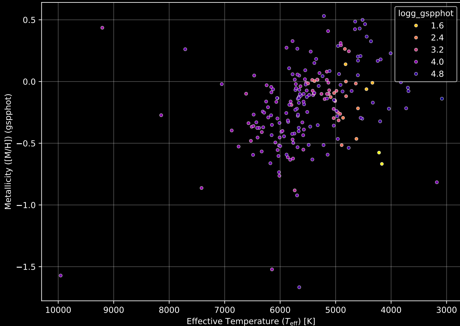
APOGEE DR17 Field: [162+36_MGA] Stellar Population Parameters (n= 208)
