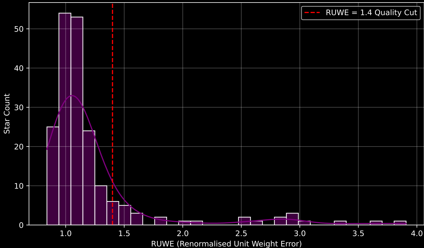
GAPOGEE DR17 Field [162+36_MGA] RUWE Distribution (n= 196)
