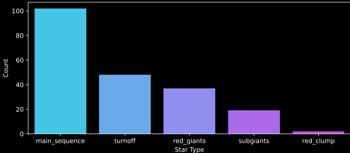
APOGEE DR17 Field: [162+36_MGA] Count plot of Star Type
