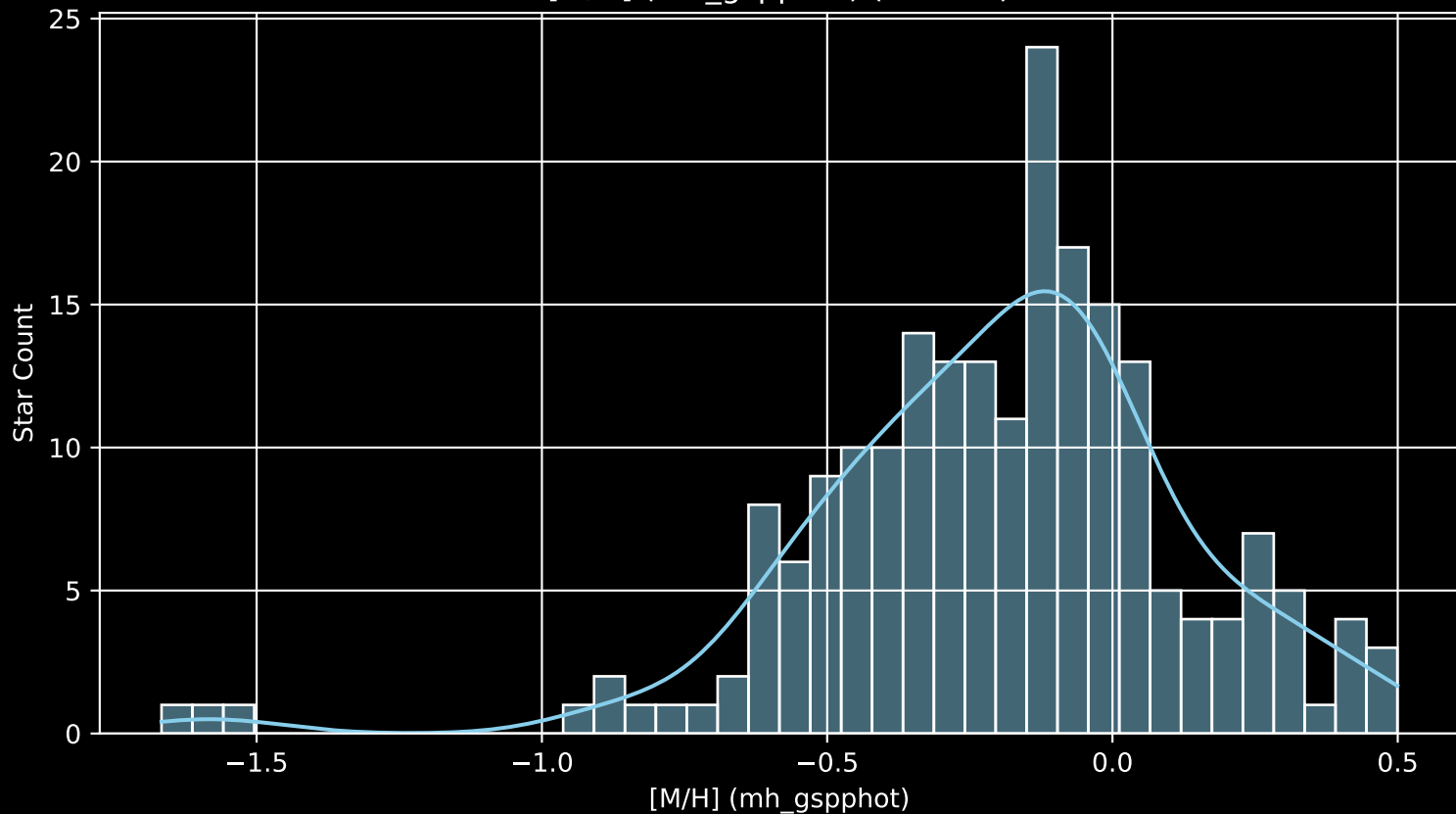
APOGEE DR17 Field: [162+36_MGA [M/H] (mh_gspphot) (n= 207)
