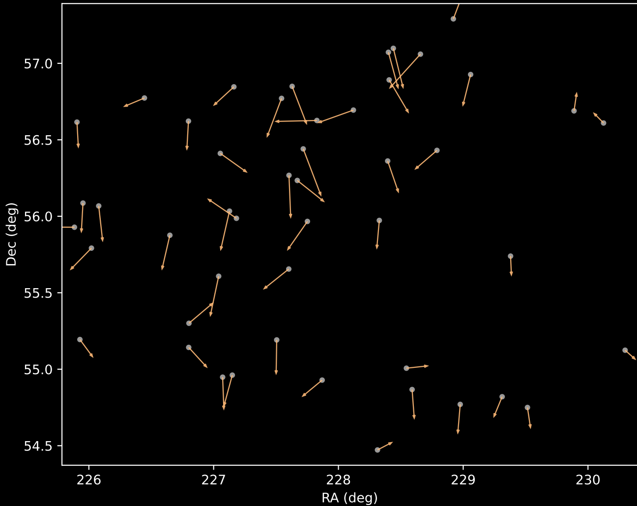
APOGEE DR17 Cluster 3 Proper Motion Vectors (n=48)
