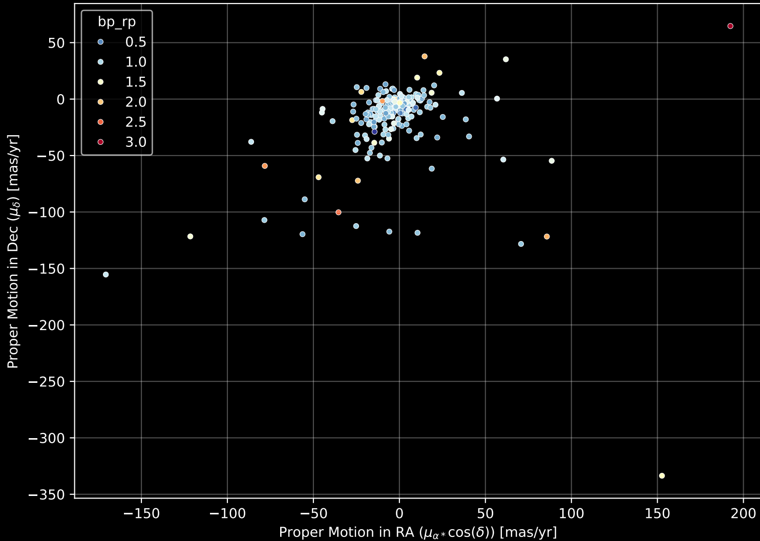
APOGEE DR17 Field: [162+36_MGA] Proper Motion Diagram (n= 208)
