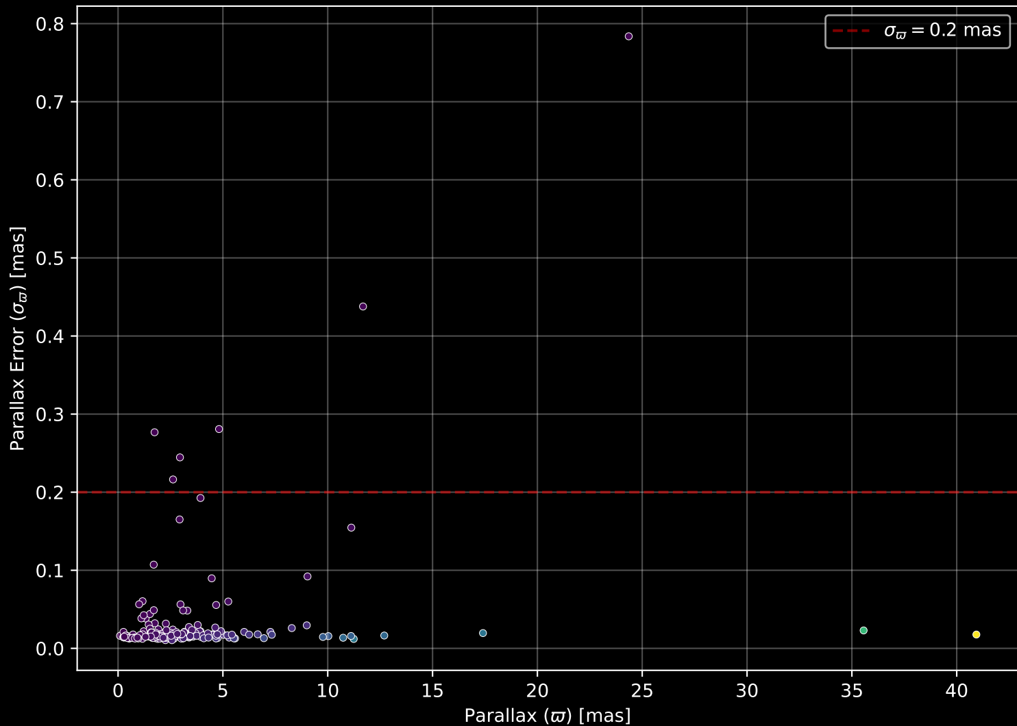
APOGEE DR17 Field: [162+36_MGA] Parallax Quality (n= 208)
